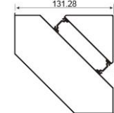
XTC-ZJ130A 130 corner -90° Weight: 2.80kg/m
