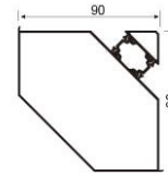
XTC-ZJ90A 90 corner -90° Weight: 1.728kg/m
