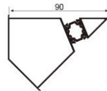
XTC-ZJ90B 90 corner -135° Weight: 1.251kg/m
