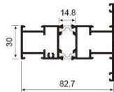
JNW-CT1343G four-rail center column Weight: 1.54kg/m
