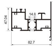
JNW-CT1346F four-rail bottom rail Weight: 1.80kg/m
