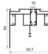
JNW-CT1487F four-rail top rail Weight: 2.32kg/m
