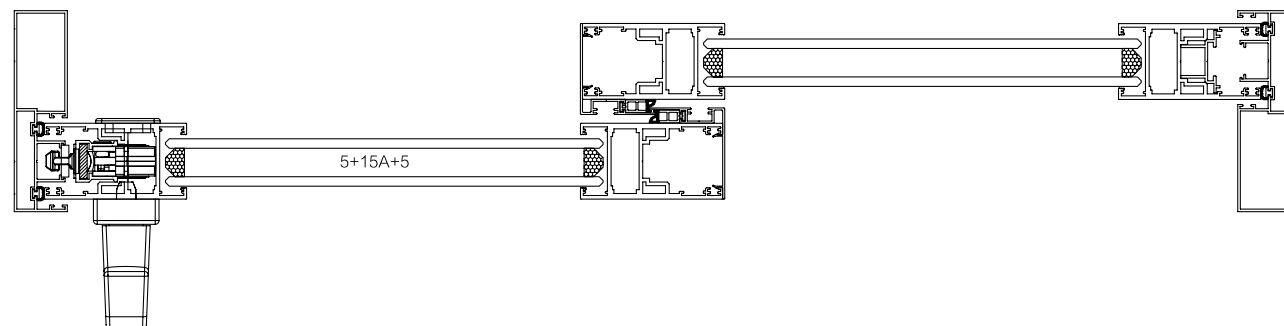
2 Tracks, 2 Panels
