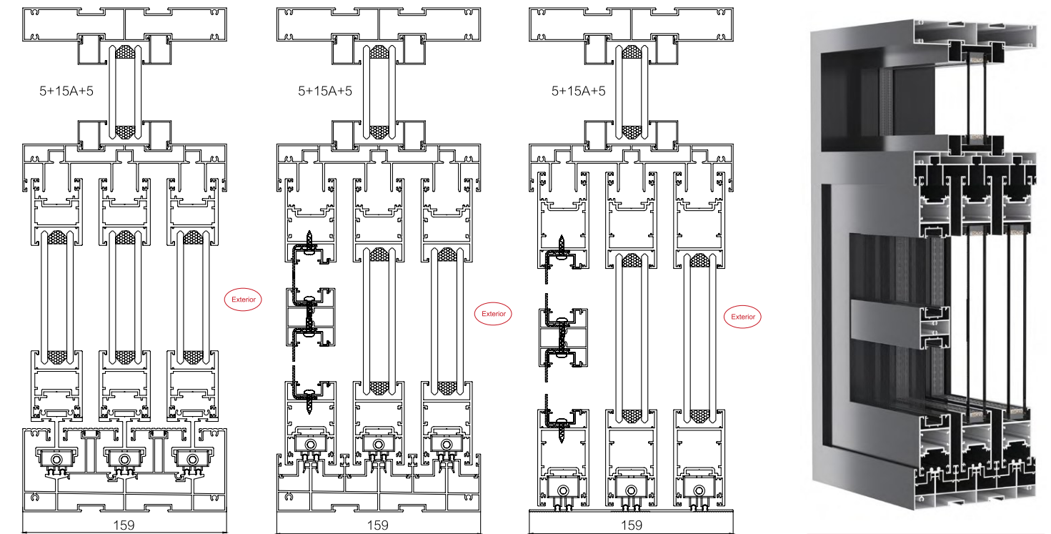
65 mm Sash - High Track
