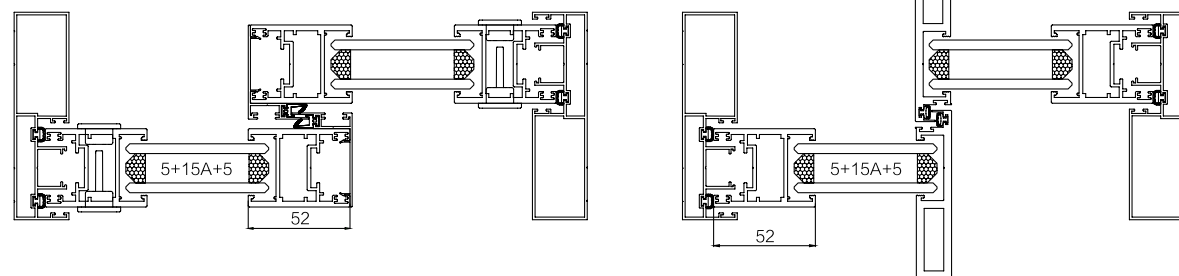
2 Tracks, 4 Panels
