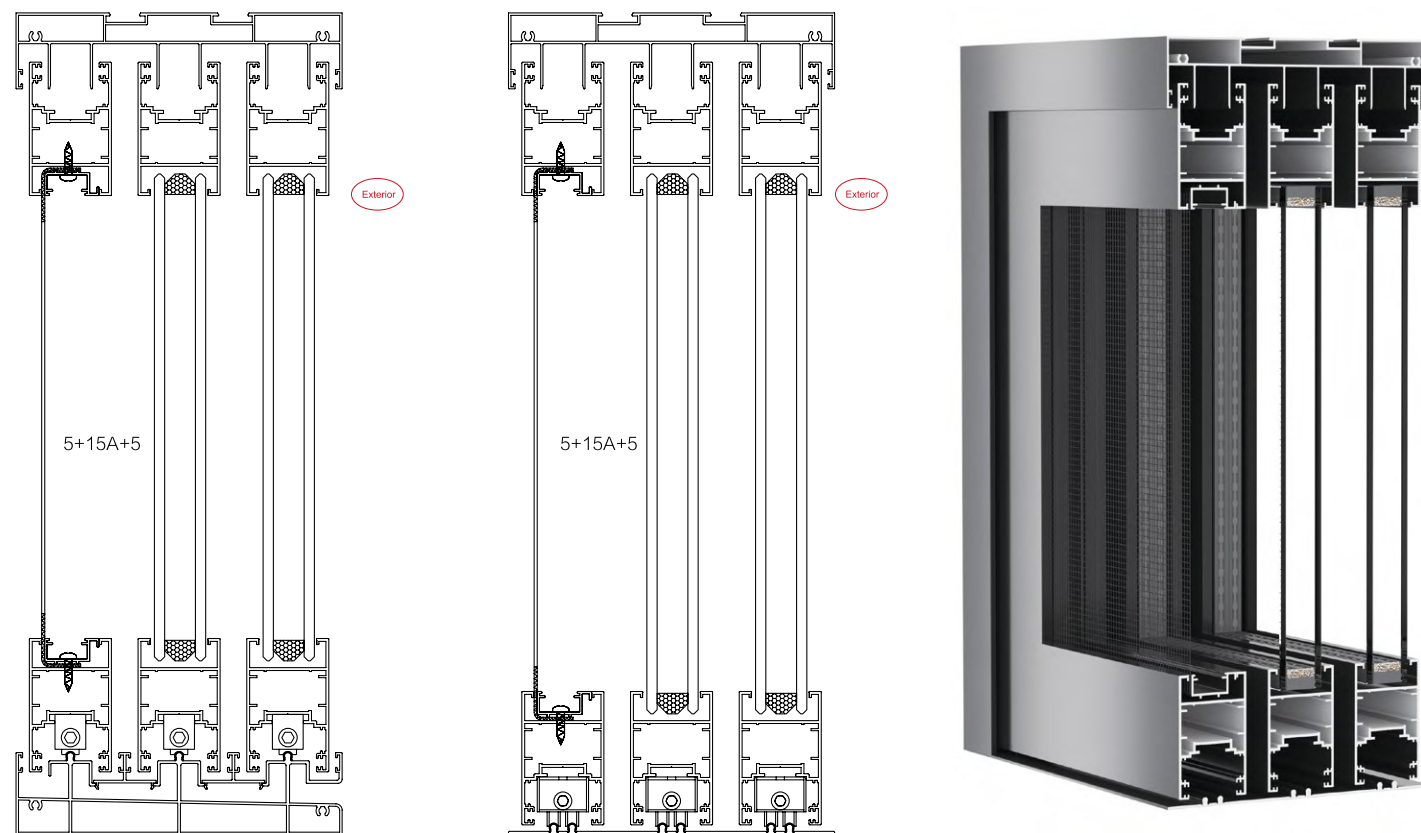
Triple Tracks Assemble Diagram
