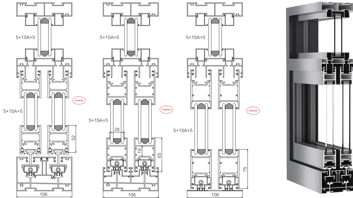
52 mm Sash - Floating Track
