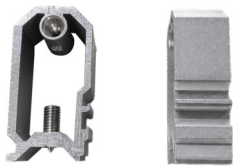
KY01 - Plain-Stile Corner Cleat for 65/75 mm Wide-Narrow Configuration (29.7ZH x 18.6)
