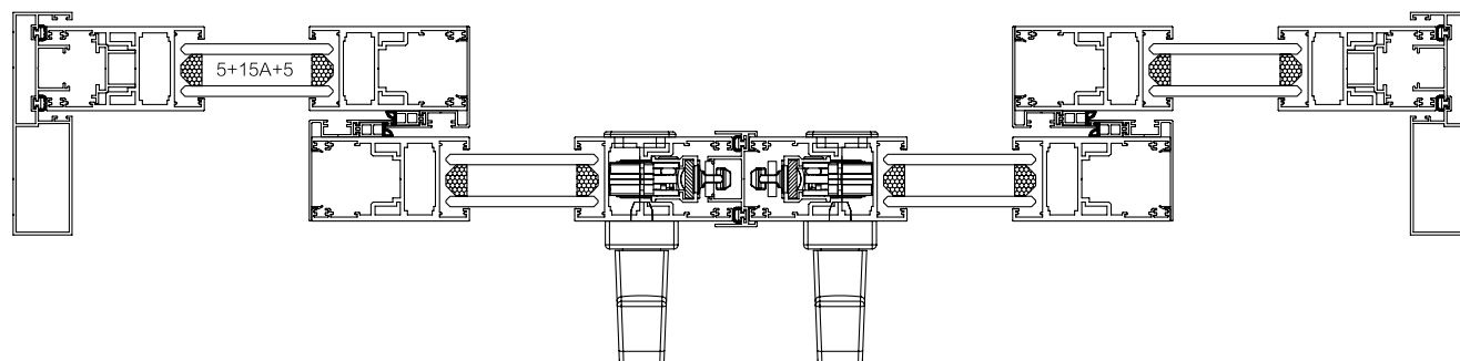
2 Tracks, 4 Panels
