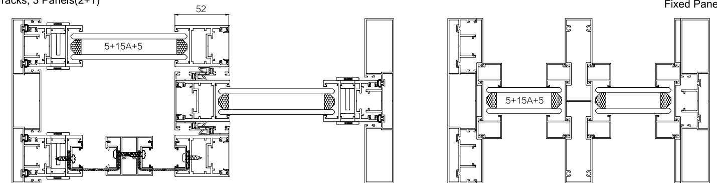
3 Tracks, 3 Panels(2+1)
