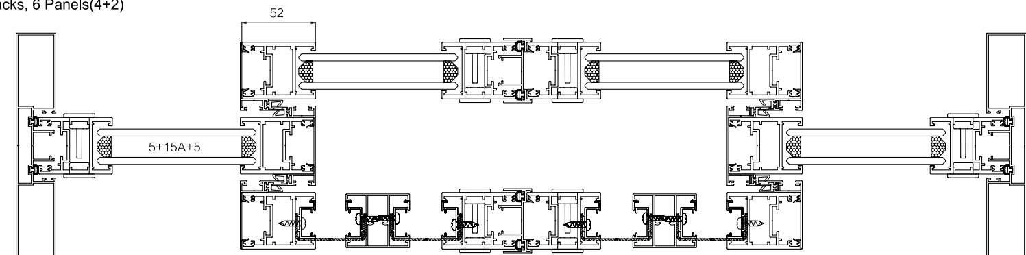
3 Tracks, 6 Panels(4+2)
