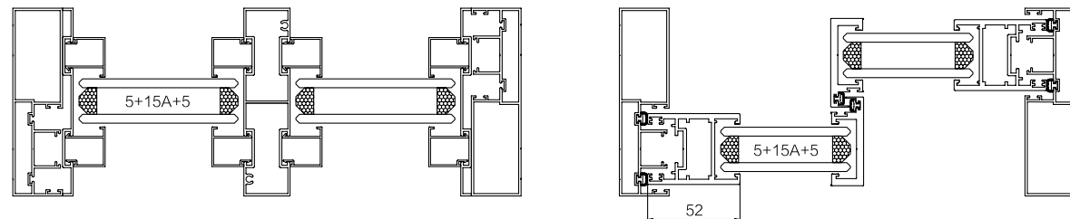
Fixed Panel
