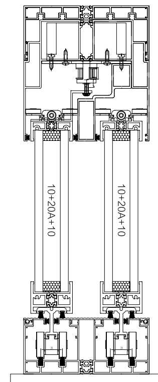
Double-Track automatic System
