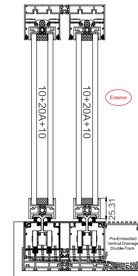
Pre-Embedded with Vertical Drainage Double Tracks
