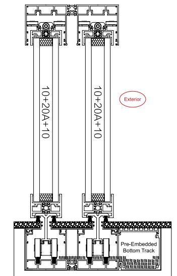
Pre-Embedded with Tile Cover Double Tracks
