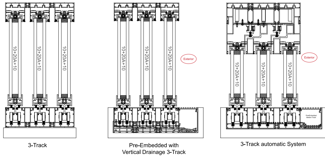
235 Panoramic Sliding Door, 3-Track 3-Panel + Security Mesh
