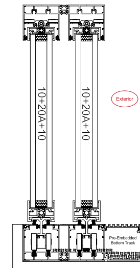
Pre-Embedded Double Tracks
