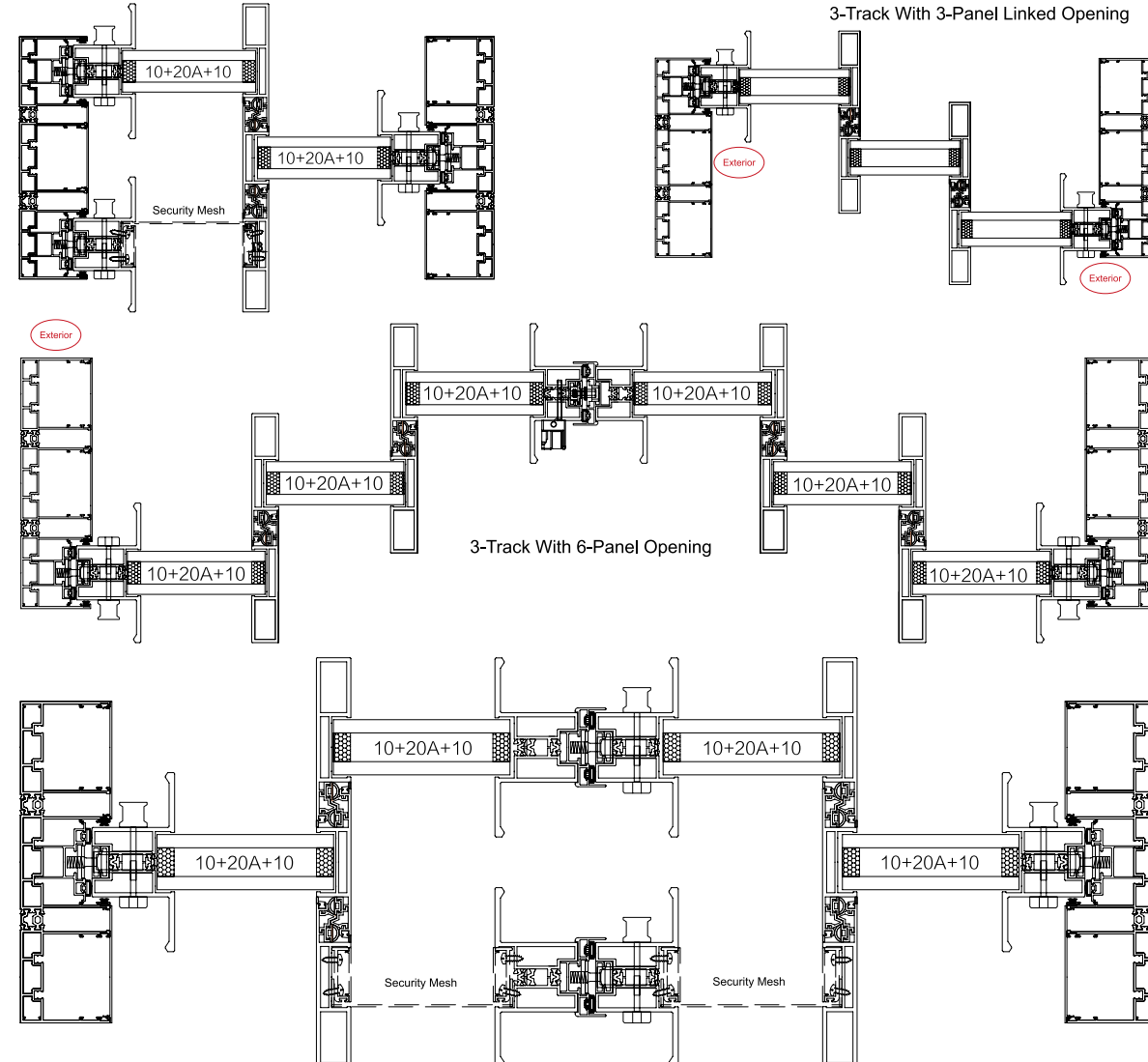
235 Panoramic Sliding Door, 3-Track 3-Panel + Security Mesh
