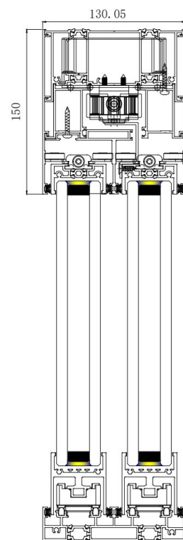
Dual-track electric - lower high track
