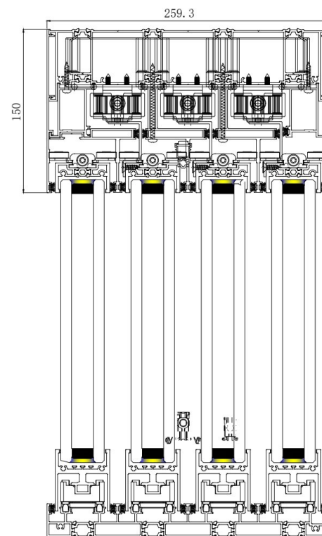
Four-track electric - lower high track
