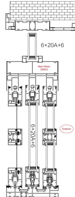
3-Track automatic System
