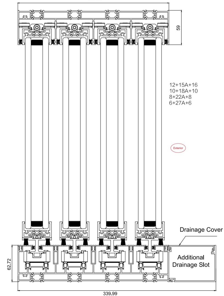
Floating Bottom Track Assembly Drawing 259.24
