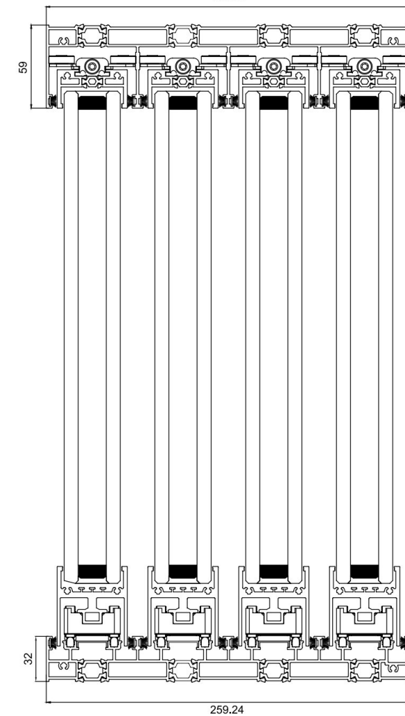
High Bottom Track Assembly Drawing 259.24
