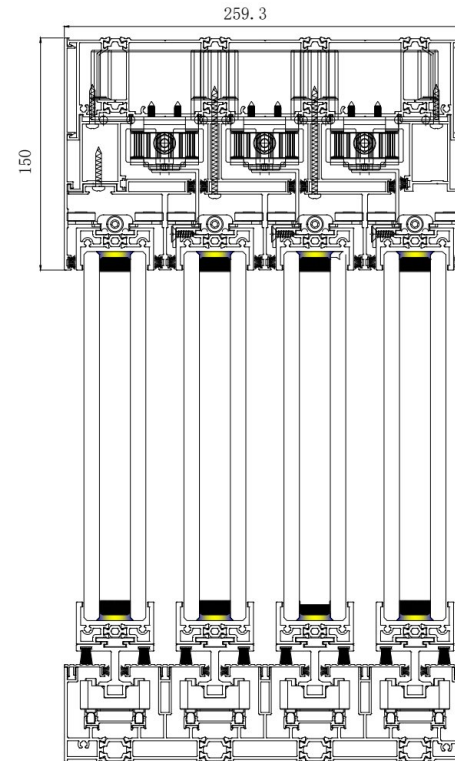
Four-track electric - lower suspended rail
