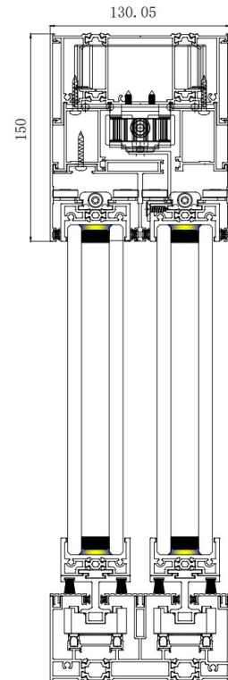
Dual-track electric-lower suspended track
