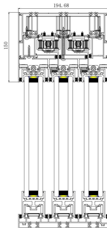
Three-rail electric - lower high rail
