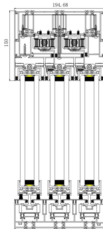
Three-rail electric - lower suspended rail
