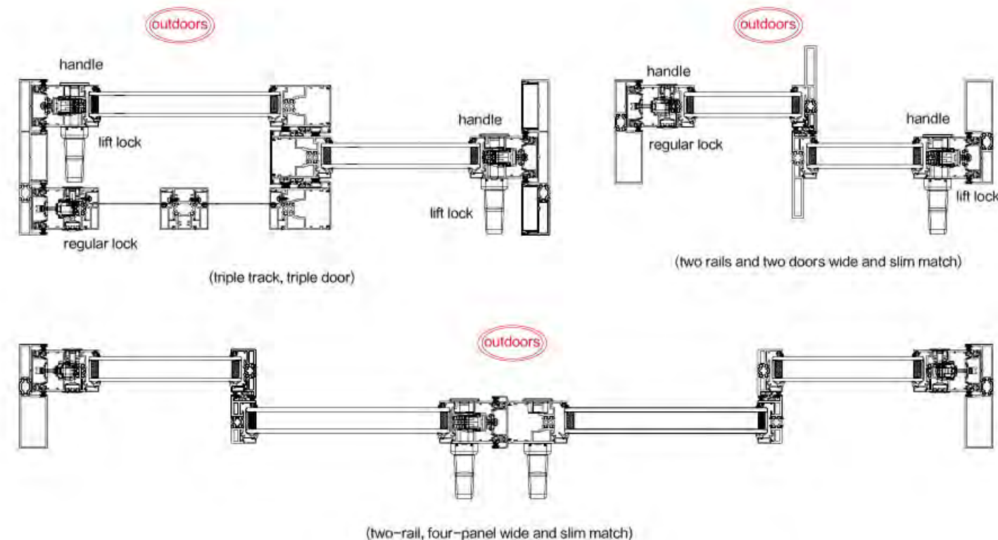
Triple track
