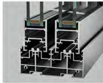
double rails higher rail double-row wheel
