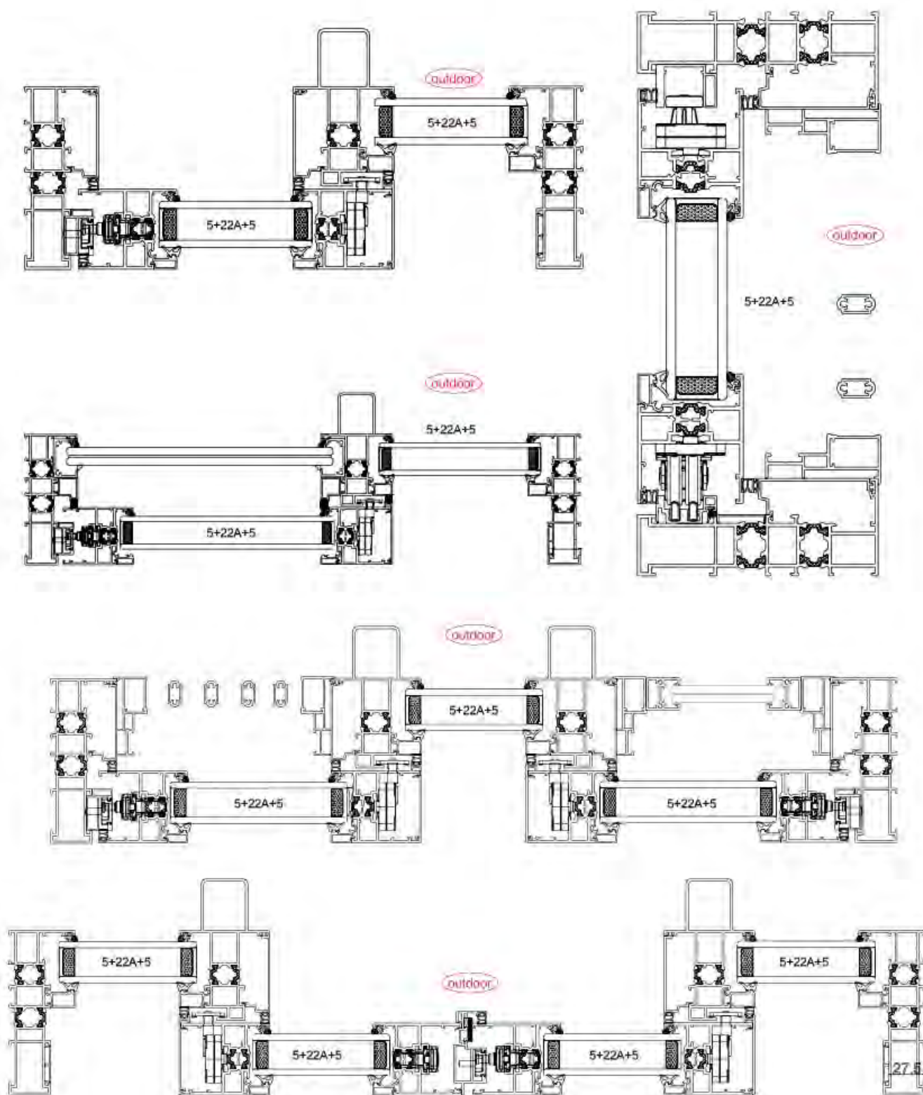
126 side pressure door
